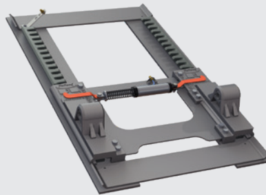
Inboard Mount
