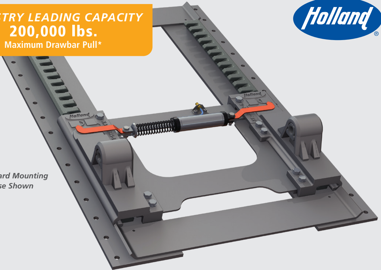
Inboard Mount
